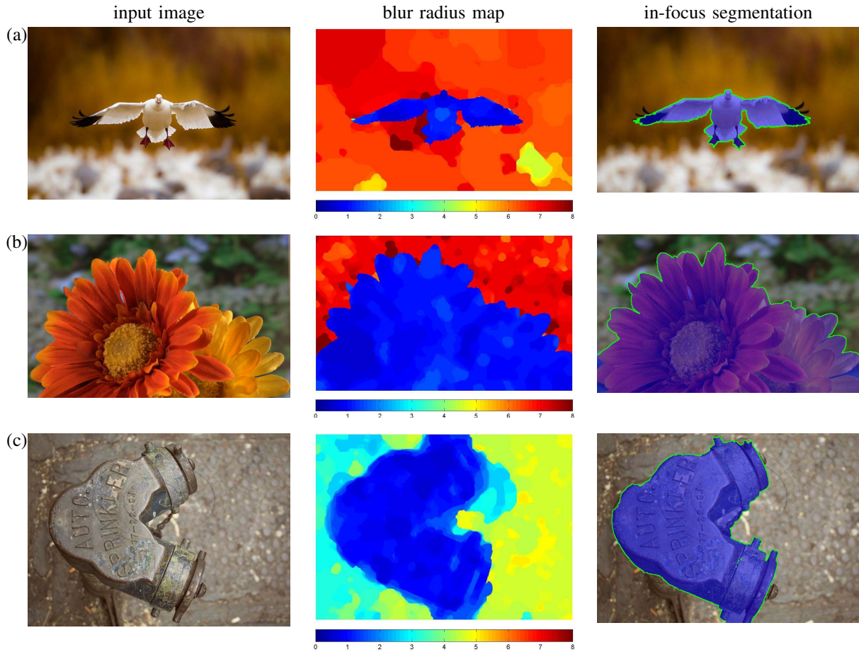
Fig. 10. More blur map results on real images. (a) bosque-Edit_small . ©Aravind Krishnaswamy. Used with permission. (b) input_training_lowres/GT01 [13]. \sigma_n^2 = 10^{-6} . (c) autoSprinkler . Image courtesy of Katrin Eismann. Segmentation based on color would be difficult in this example.
