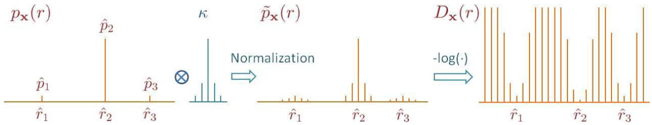
Fig. 7. Making the artificial likelihood array.
